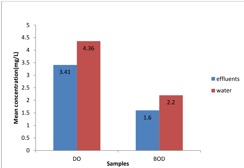
Figure 4; Monthly mean of DO and BOD of effluents and lagoon water
